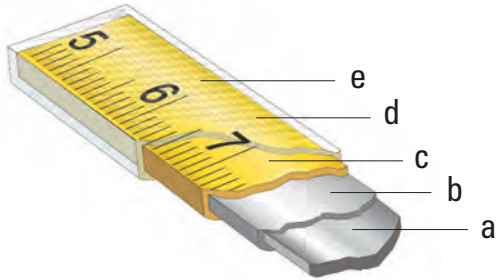
BLADE STRUCTURE OF KOMELON LONG STEEL TAPES
