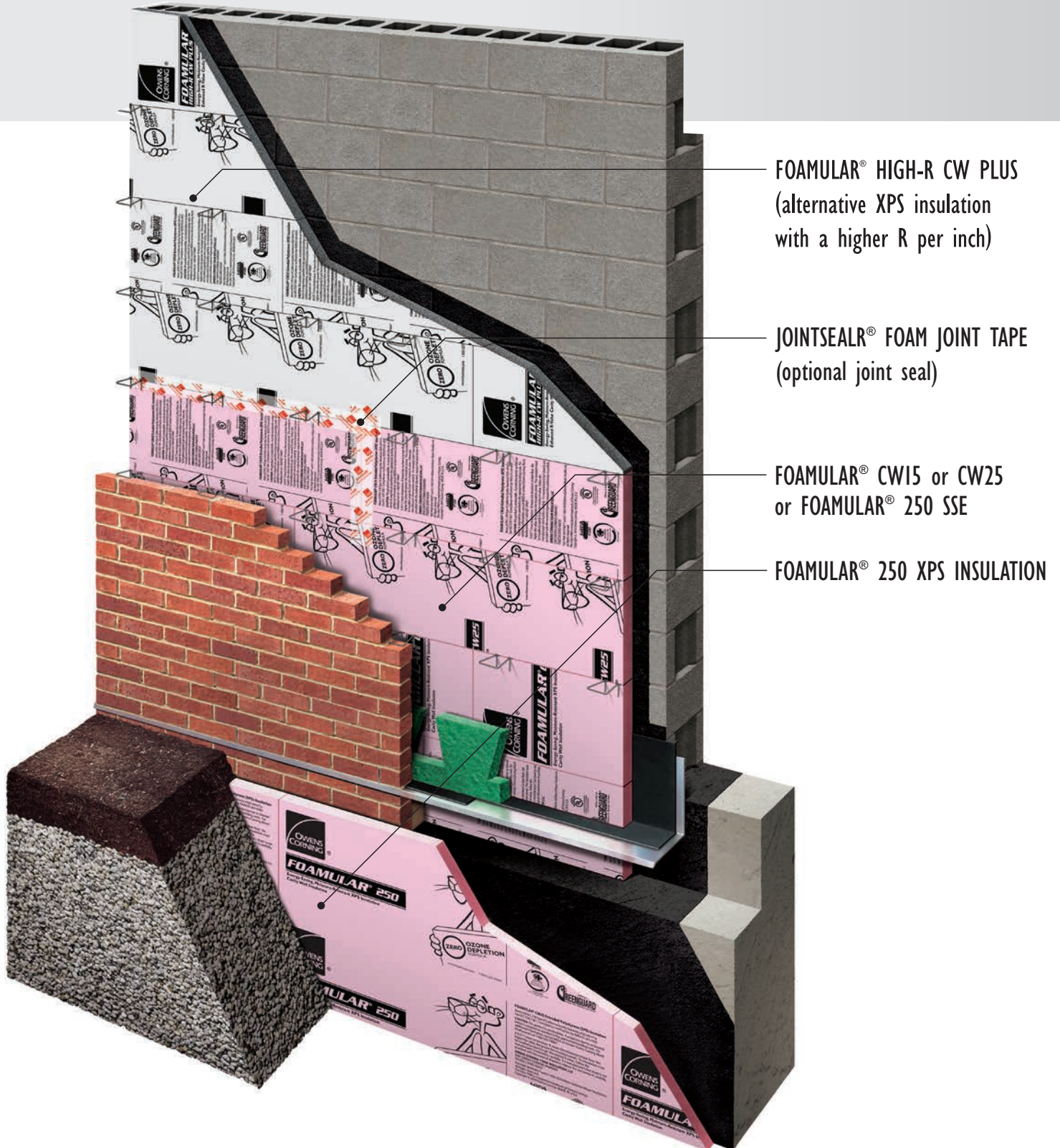
Brick, CMU, Stone, or Terra-Cotta Veneer over CMU
