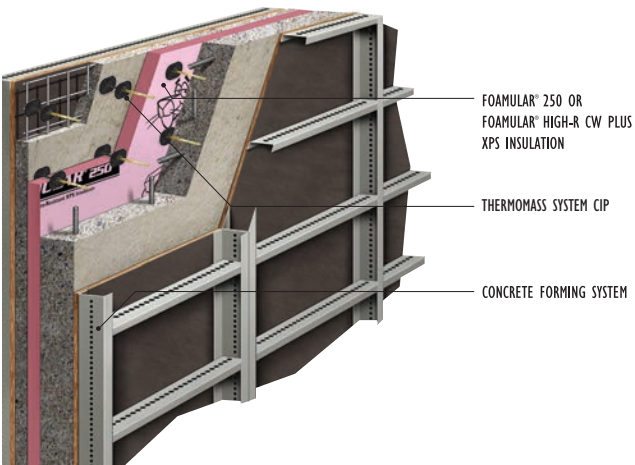
Insulated Concrete Sandwich Panel, Cast-in-Place
