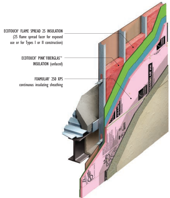
PM EIFS over Steel Stud Framing or CMU (EIFS system by others)
