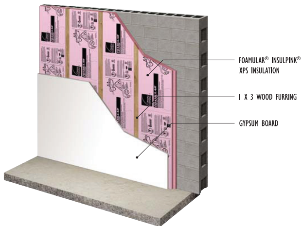
Masonry Wall with Wood Furring
