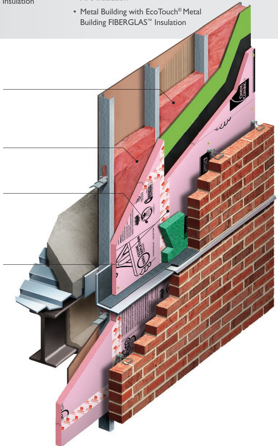
Brick, CMU, Stone, or Terra-Cotta Veneer over Steel Stud Framing
