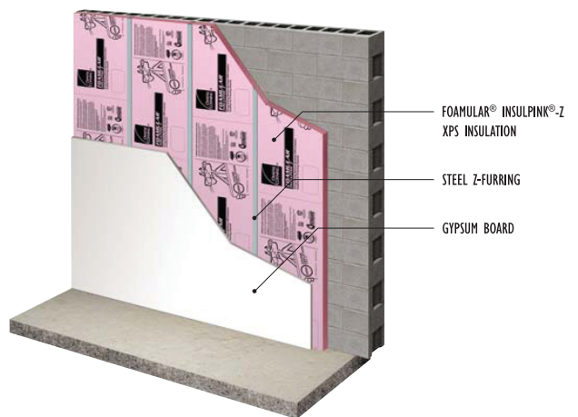
Masonry Wall with Z-Furring
